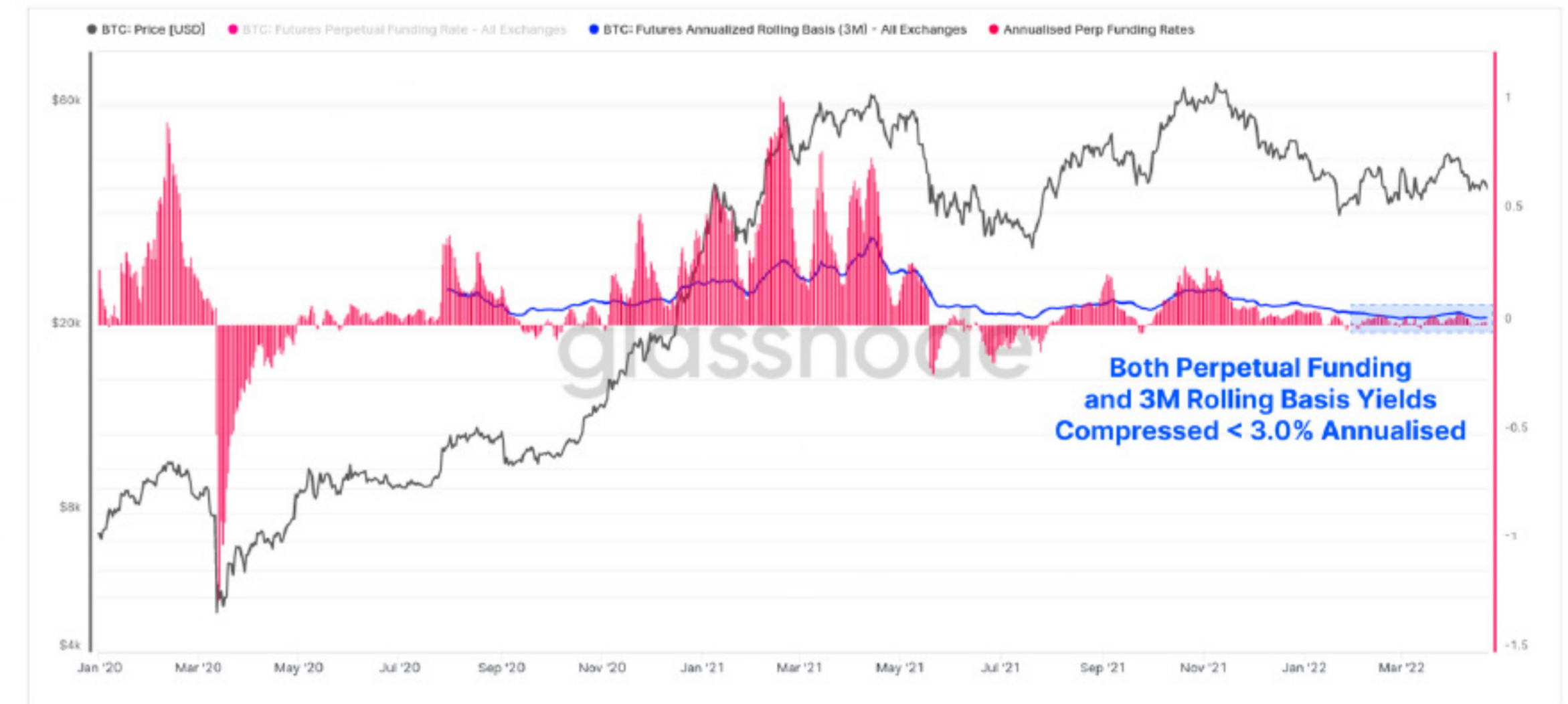
Bitcoin: Annualized Perpetual Funding vs 3m Basis
